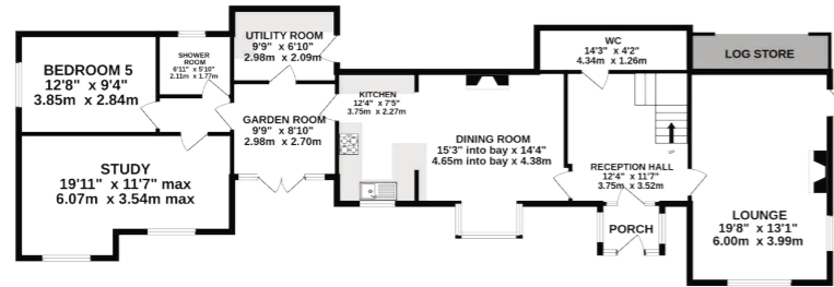
GROUND FLOOR 1297 sq.ft. (120.5 sq.m.) approx.
